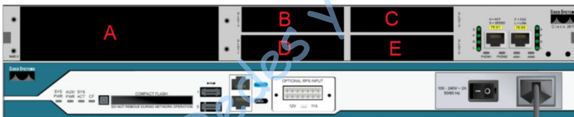
Figura No. 12. Slots del router 2811 IOS15
